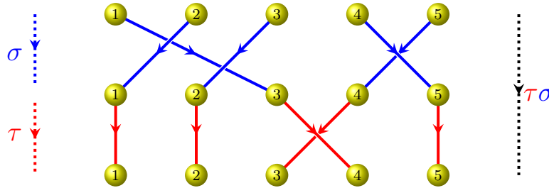
FIGURE 1.4 – Composition de permutations
